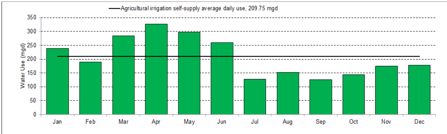
Figure 7. Average daily agricultural self-supply freshwater use (mgd) by month, 2021
