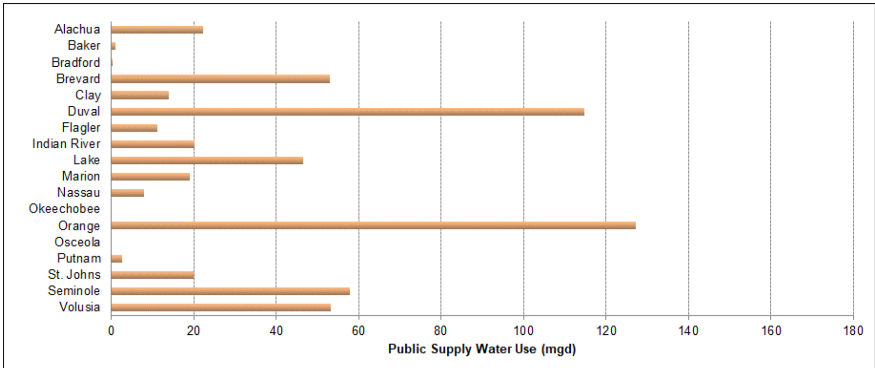
Figure 4. Water use (mgd) for public supply in SJRWMD, 2021
