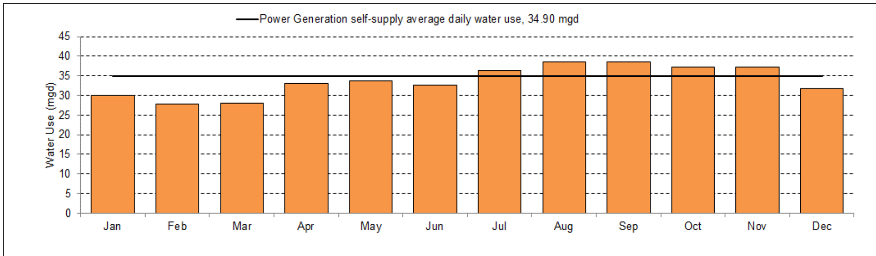
Figure 10. Average daily power generation self-supply freshwater use by month, 2021
