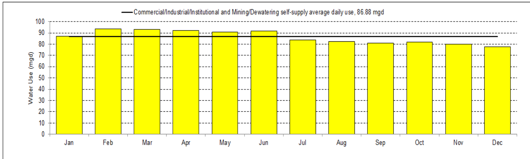
Figure 6. Average daily commercial/industrial/institutional and mining/dewatering self-supply freshwater use (mgd) by month, 2021
